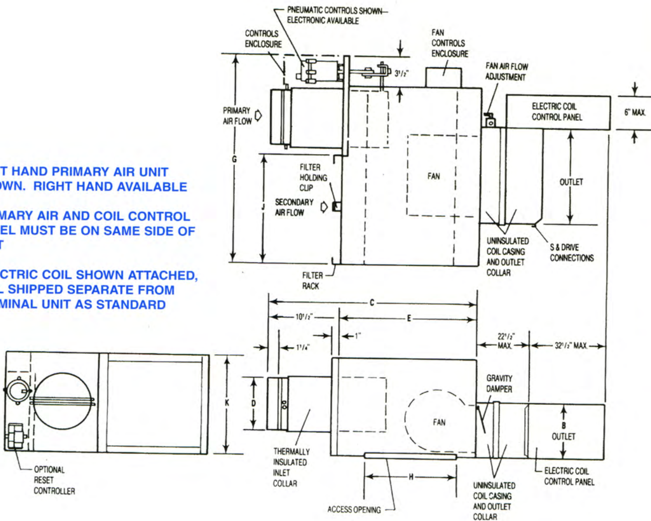
DIMENSIONS LISTED IN INCHES
