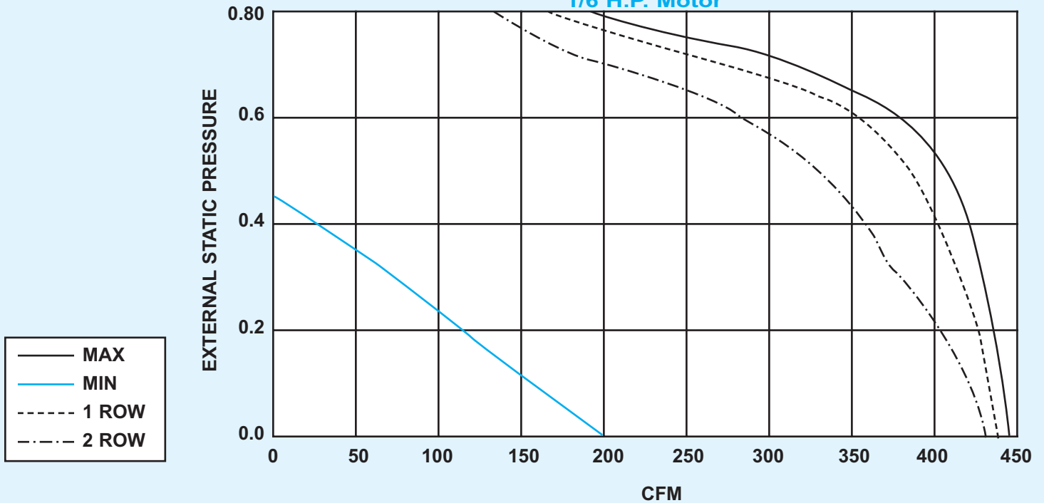
FAN SIZE B - AS L2, L3, L4 1/6 H.P. Motor
