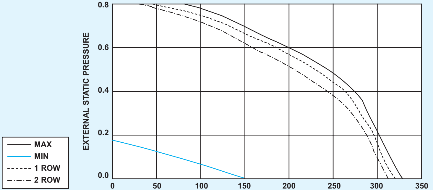
FAN SIZE A - AS L1, L2, L3 1/6 H.P. Motor
