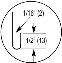
RECOMMENDED DUCT HEM DIMENSIONS
