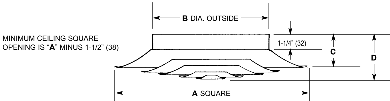
DIMENSIONS LISTED IN INCHES (Millimeters)
