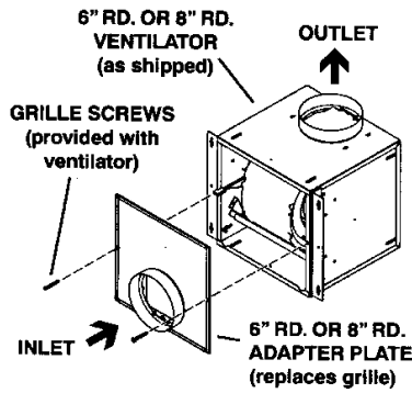
6" ROUND & 8" ROUND VENTILATOR Right Angle Discharge
