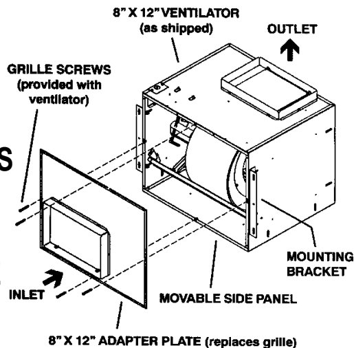
8" X 12" VENTILATOR Right Angle Discharge
