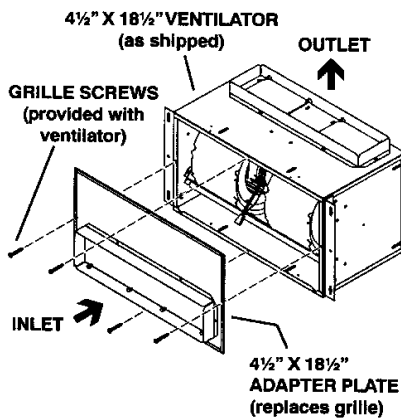
4 1/2" X 18 1/2" VENTILATOR Right Angle Discharge
