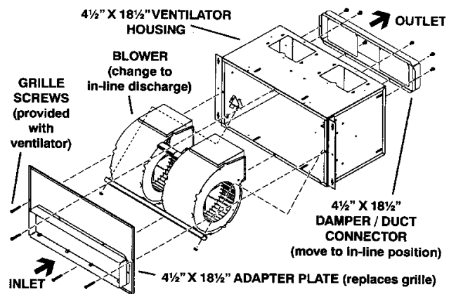
4 1/2" X 18 1/2" VENTILATOR Straight-Through Discharge
