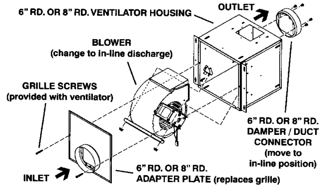
6" ROUND & 8" ROUND VENTILATOR Straight-Through Discharge
