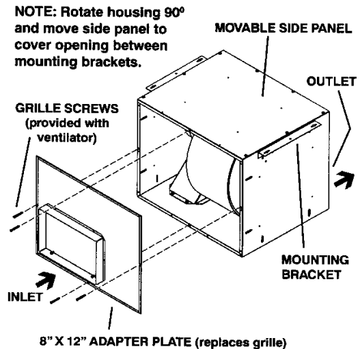
8" X 12" VENTILATOR Straight-Through Discharge
