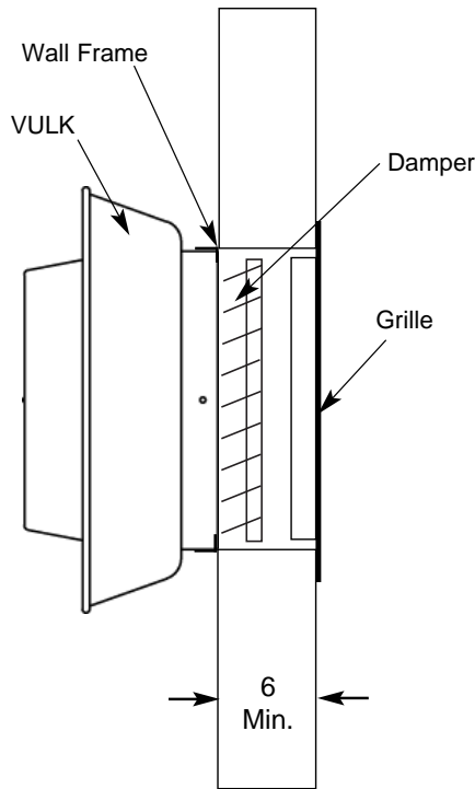
Figure 5 NON-DUCTED Sidewall Installation
